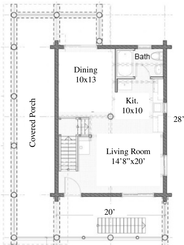
First Floor 560 sq. ft.
