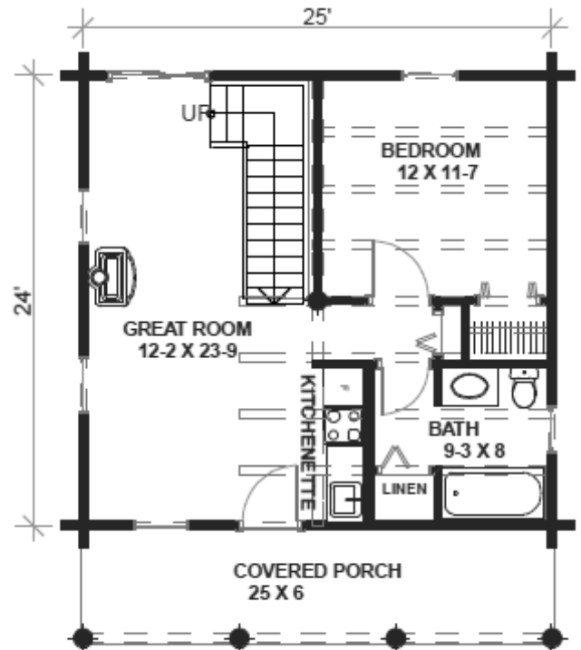
MAIN FLOOR 616 sq. ft.
